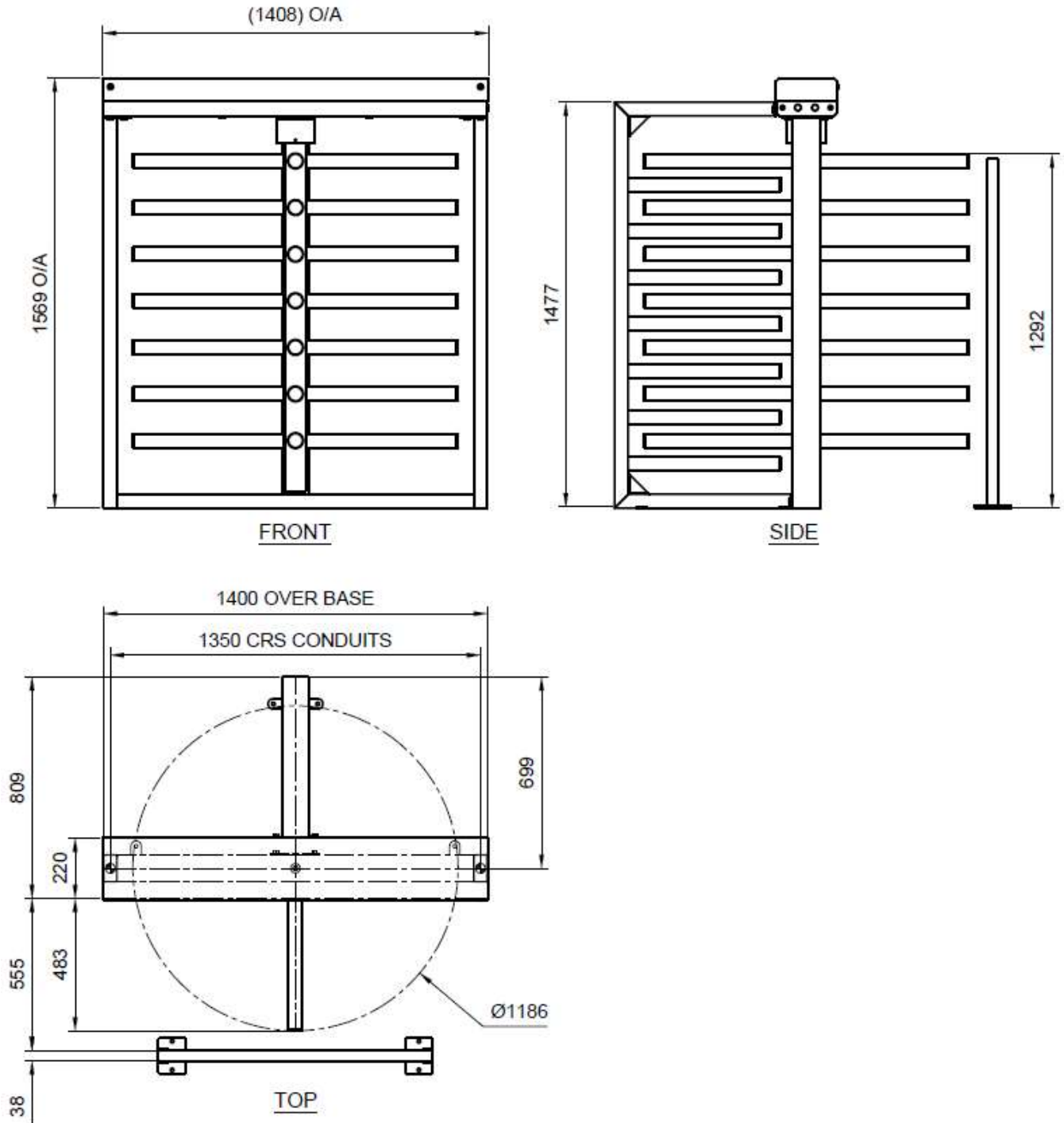
Figure 5: Single 4-Arm Industrial 3/4 Height Turnstile
