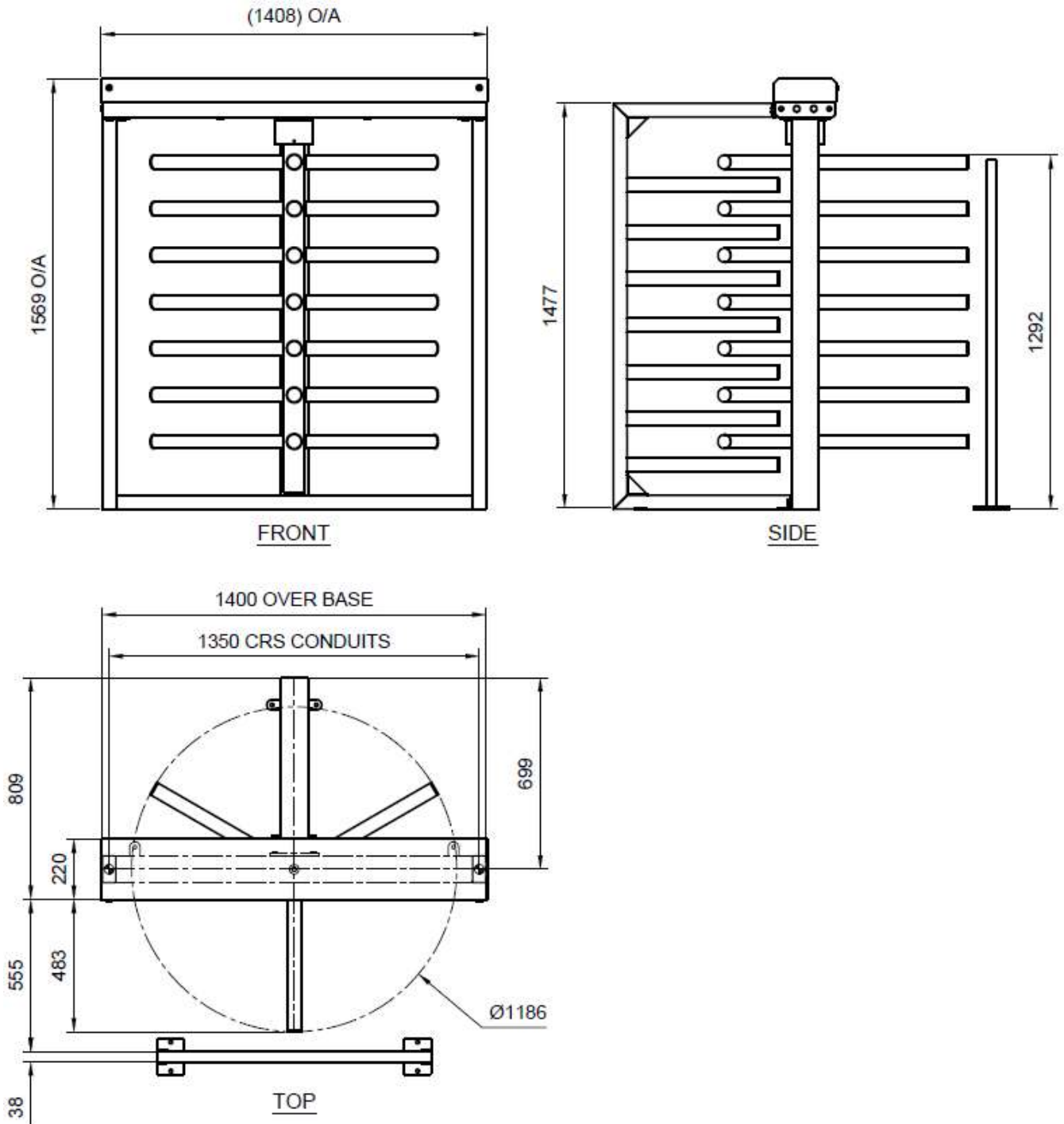
Figure 6: Single 3-Arm Industrial 3/4 Height Turnstile
