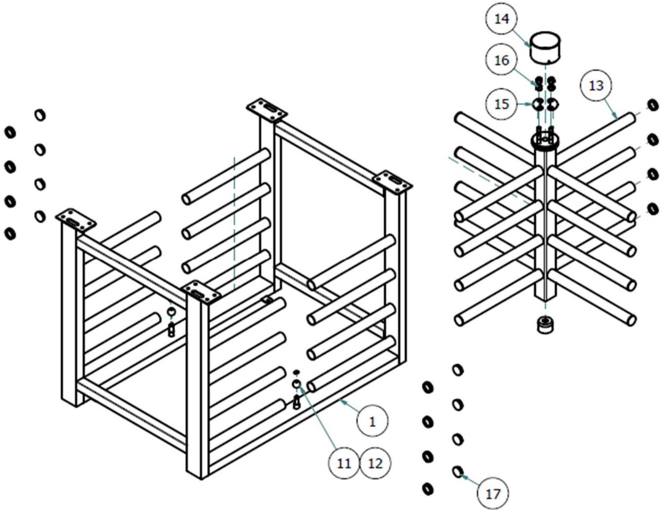
Figure 18: Double Turnstile Exploded Parts 2
