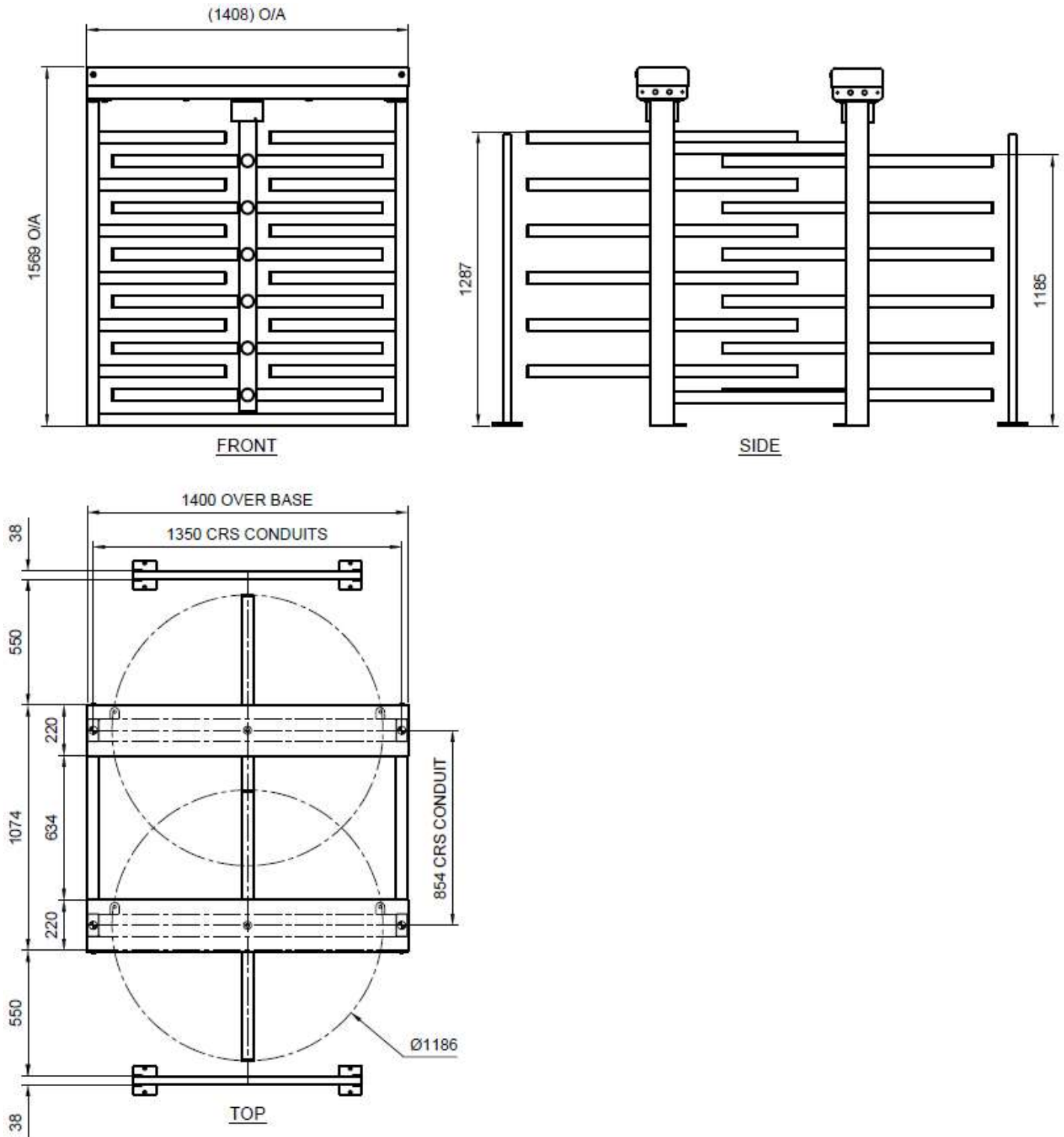
Figure 7: Double 4-Arm Industrial 3/4 Height Turnstile
